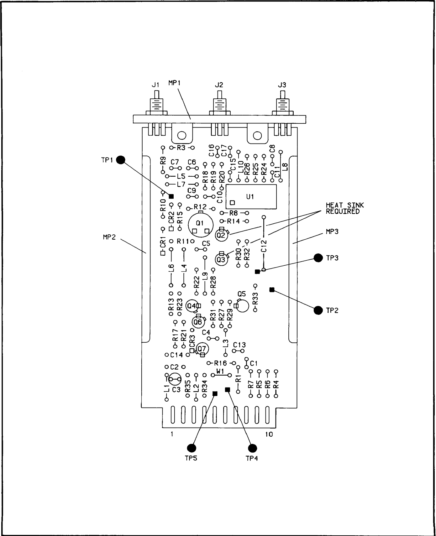
Figure 8-440. A3A9 FM Sum Loop Mixer Component Locator
