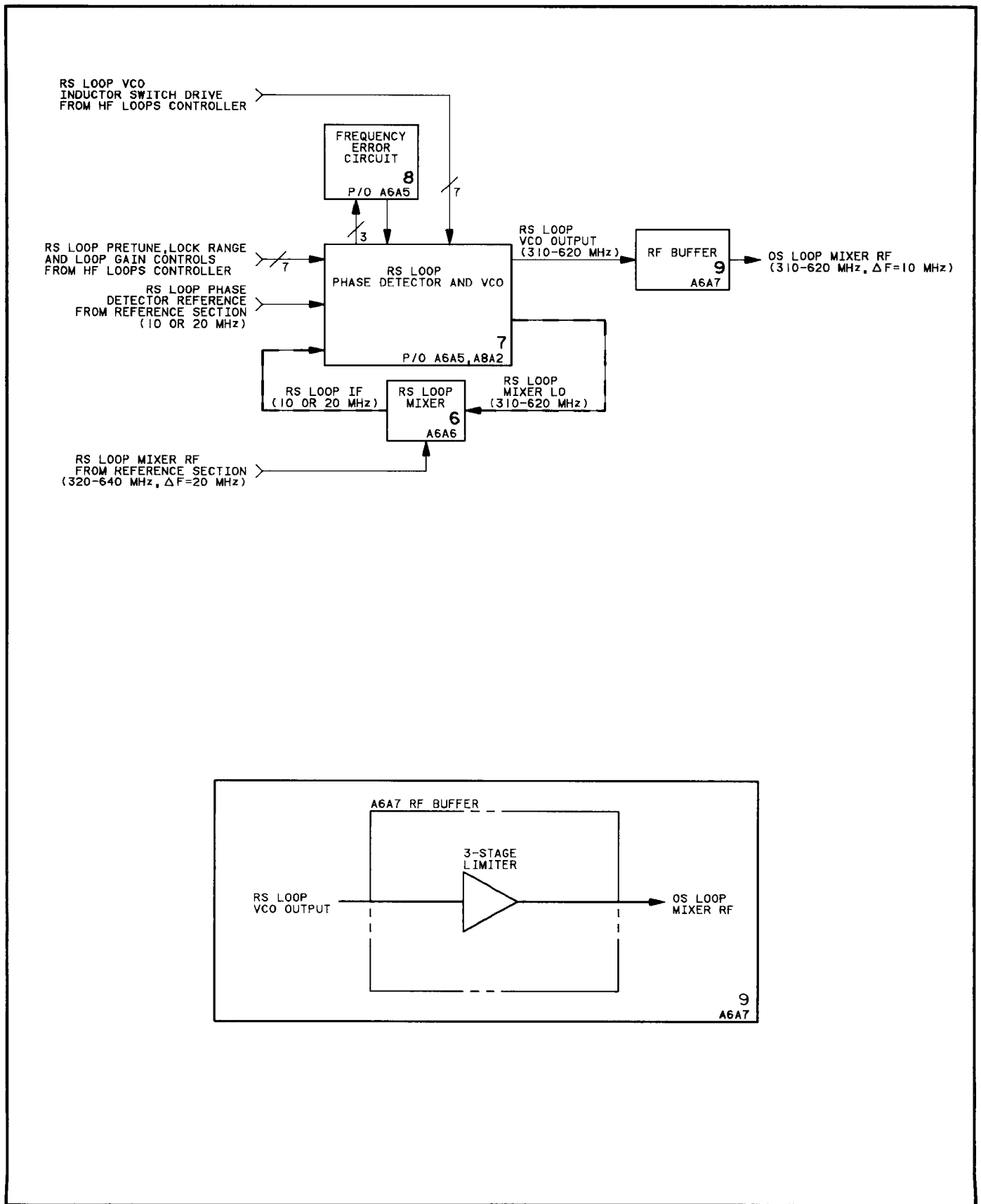
Figure 8-325. A6A7 RF Buffer Block Diagrams
