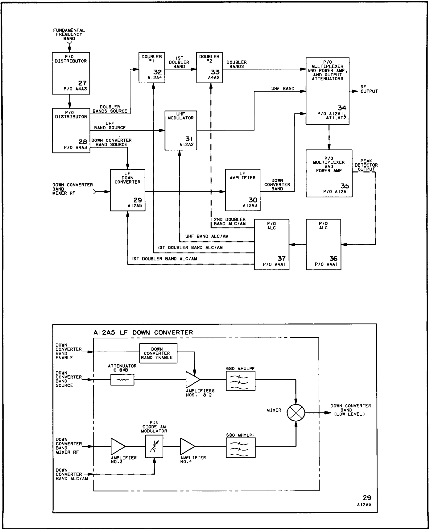
Figure 8-507. A12A5 LF Down Converter Block Diagrams
