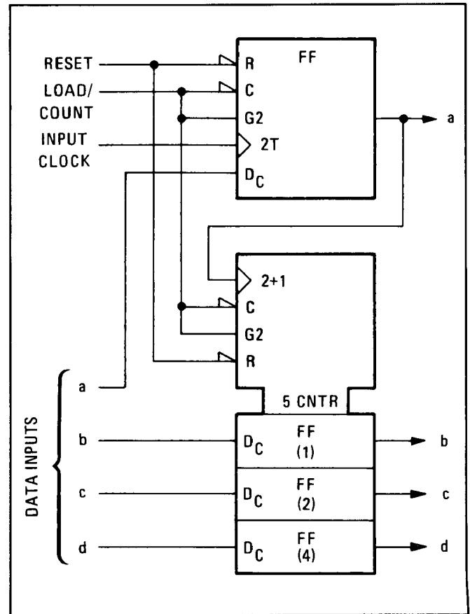
Figure 8-118. Presetable Counter
