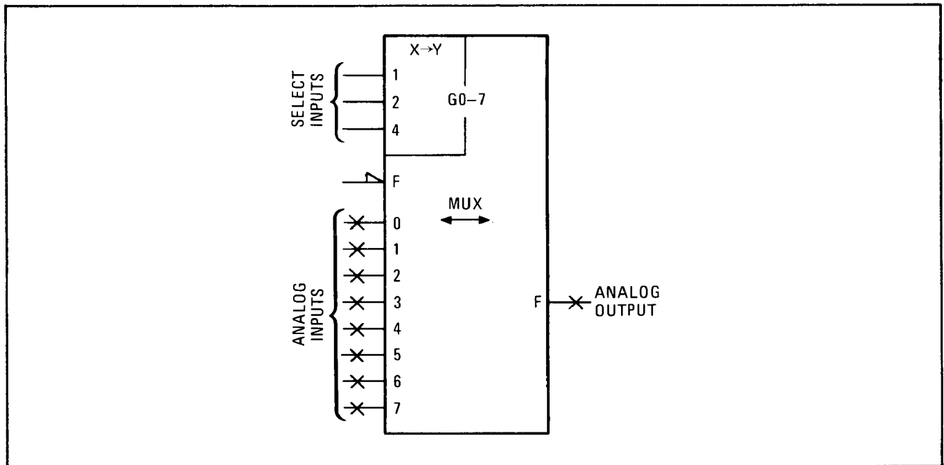
Figure 8-128. Analog Multiplexer
