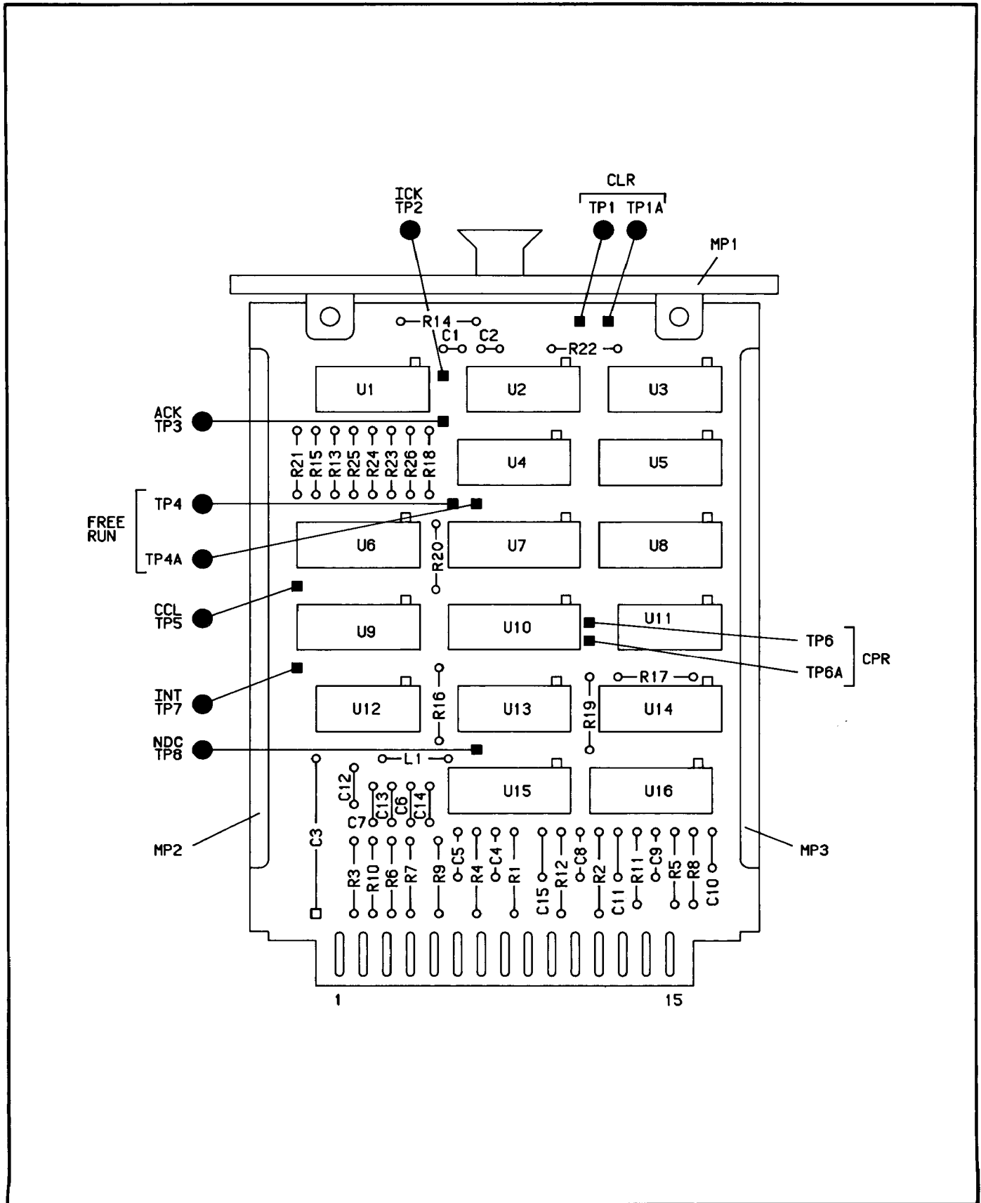
Figure 8-419. A5A1 Fractional-N Loop Accumulator Component Locator
