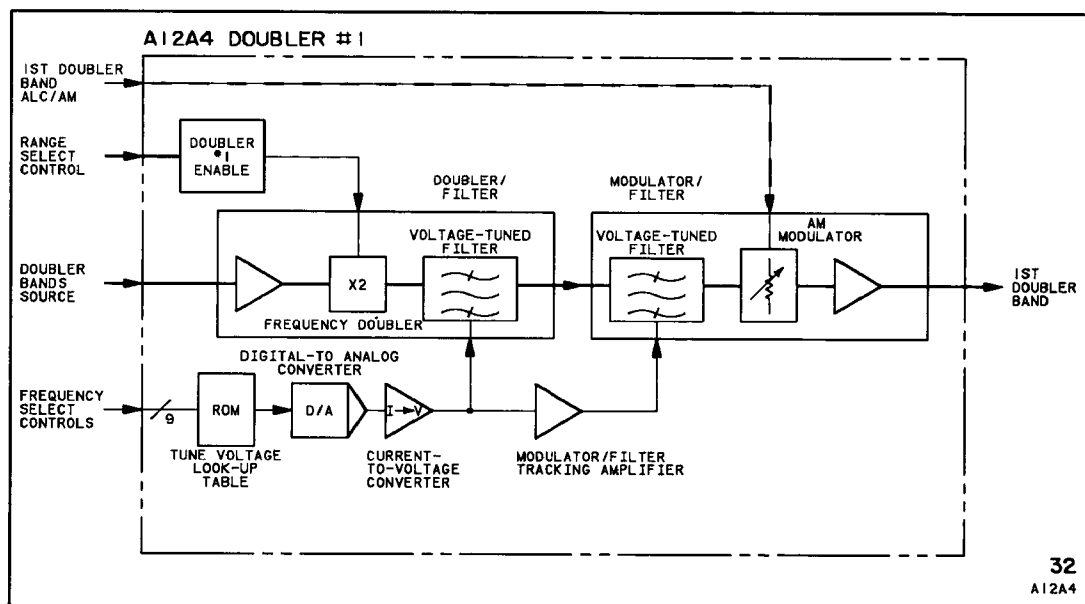
Figure 8-516. A12A4 Doublers #1 Block Diagrams
